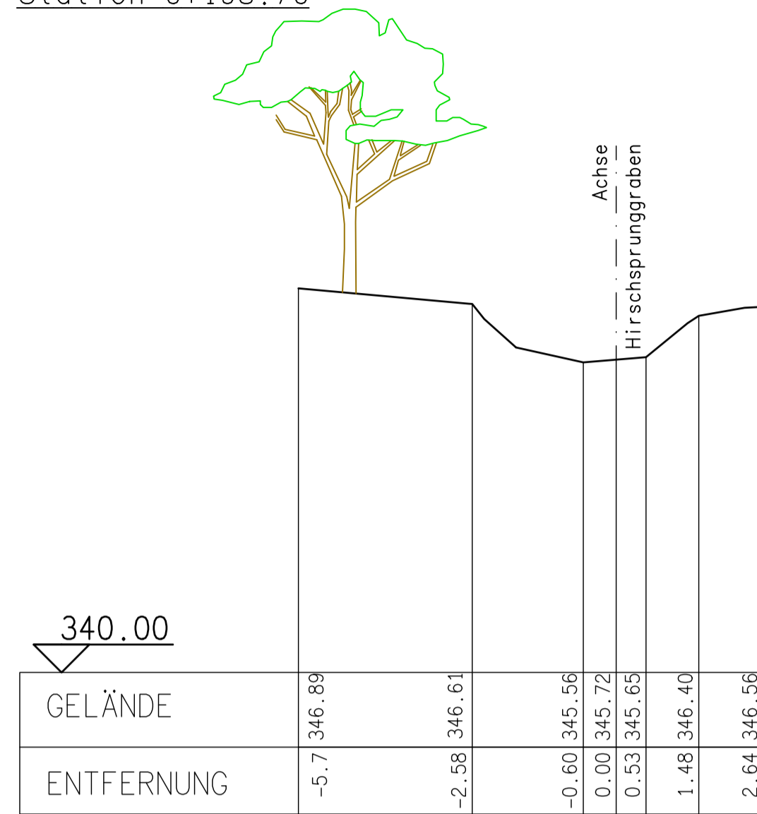
Station 0+193.70
