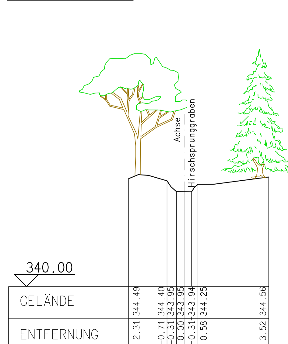
Station 0+243.70
