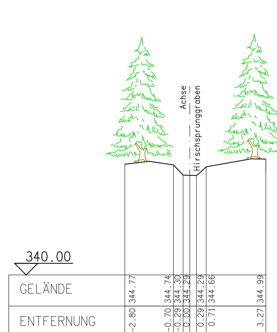
Station 0+233.70
