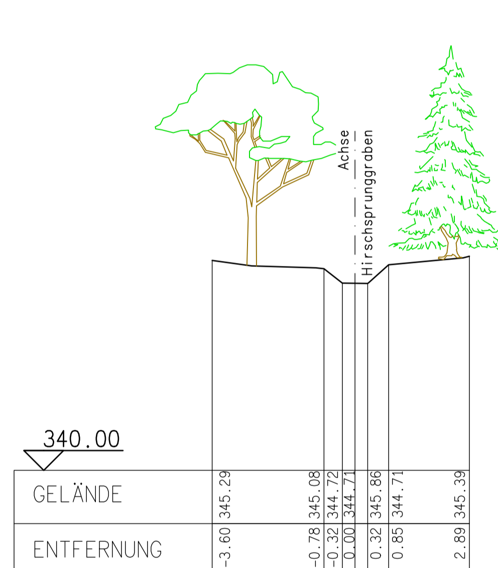
Station 0+223.70
