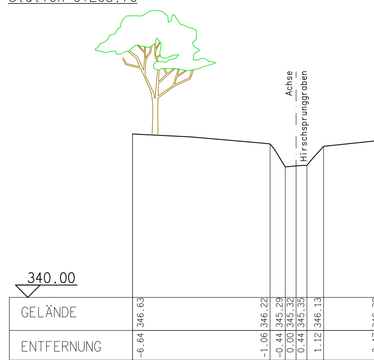
Station 0+203.70
