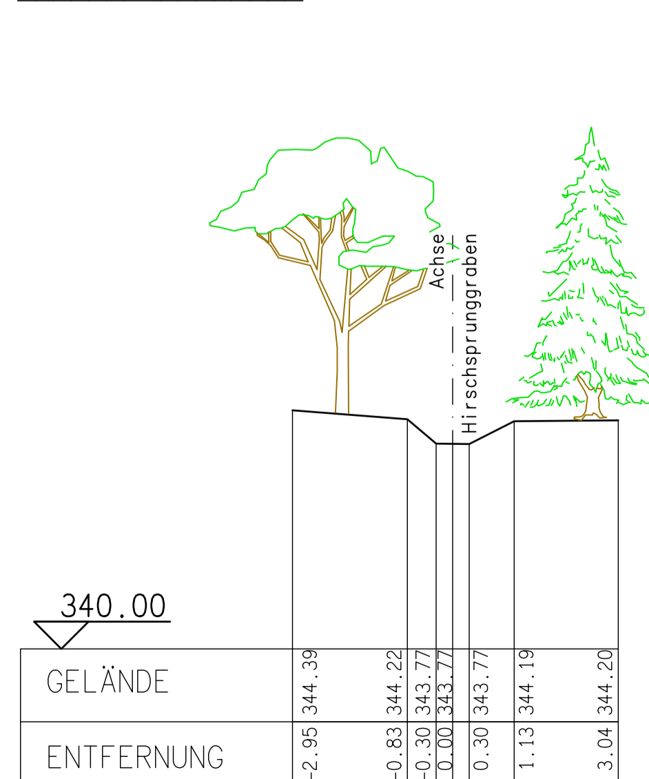
Station 0+249.58
