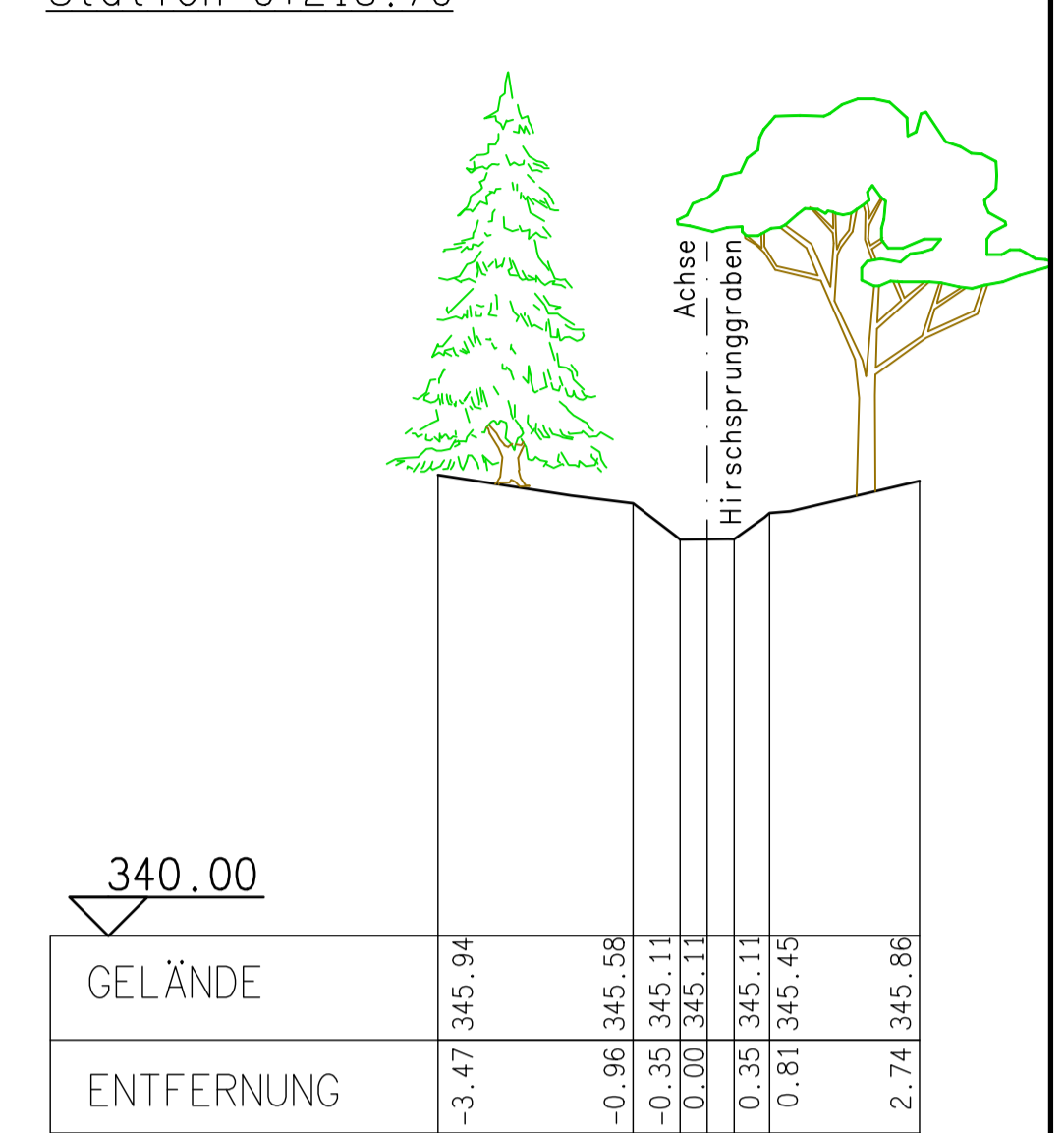
Station 0+213.70
